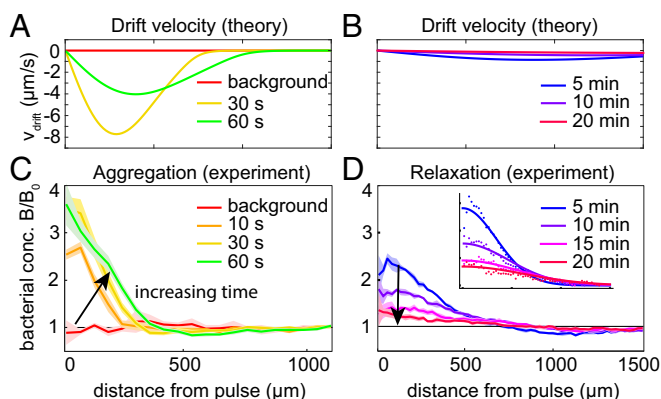
Fig. 5. Time-dependent bacterial response to photoreleased nutrients of initial concentration C_0 = 35 \mu\text{M} (mass 0.22 \text{ pmol} ). (A and B) Theoretically predicted radial velocity profiles at various times, obtained by using SI Appendix, Eq. S22 . (C) Experimental snapshots of bacterial concentration at t = 10, 30, 60 \text{ s} after creation of a diffusing nutrient pulse. Conservation of bacteria dictates that beyond the aggregation ( B > B_0 ) exists a depletion zone, where B < B_0 . (D) The bacterial concentration takes approximately 20 min to relax to B(r, t) \approx B_0 . D, Inset shows that B(r, t) for t \gtrsim 300 \text{ s} is well captured by diffusive spreading alone with a diffusion coefficient D_B = 165 \mu\text{m}^2 \cdot \text{s}^{-1} .
