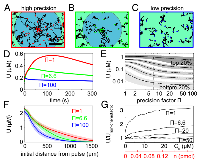
Fig. 4. (A–C) Numerical simulations of bacteria for varying values of the chemotactic precision factor ( \Pi = 1, 6.6, 100 ) show that aggregation depends strongly on chemotactic precision. Sample trajectories of 100 model bacteria followed for 60 s are shown (Movies S1–S3). The shaded circular zones (blue) represent a measured drift velocity |v_{\text{drift}}| > 1 \mu\text{m/s} over the first 60 s. (Scale bar: 500 \mu\text{m} .) (D) Nutrient exposure U as a function of time, averaged across the population. Results are shown for three different precision factors, \Pi , corresponding to those in A–C. (E) Time-averaged nutrient exposure as a function of precision for different quintiles of the bacterial population. (F) Mean nutrient exposure U as a function of the initial distance of bacteria from the pulse. Shaded regions show SE. D–F correspond to C_0 = 35 \mu\text{M} . (G) Enhancement in potential uptake compared with nonchemotactic cells as a function of pulse size.
