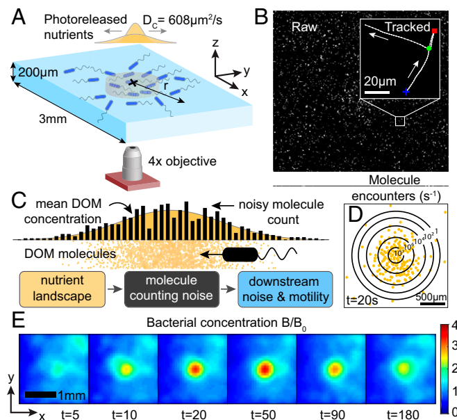
Fig. 1. Bacteria are able to perform chemotaxis in the presence of molecule counting noise. (A) Localized chemoattractant becomes available at the center of the chamber through photorelease of caged glutamate (orange), which subsequently diffuses and attracts chemotactic bacteria (blue). (B) Bacterial trajectories are extracted across the domain, revealing runs (white), reversals (red), and flicks (green). (C) The discrete nature of glutamate encounters introduces noise into the bacterium's gradient measurement on top of other sources of noise. (D) Contours showing the instantaneous rate of encounter with glutamate molecules experienced by bacteria (shown at t = 20 s). (E) Despite the noise, the cells exhibit strong accumulation with bacterial cell concentration, B/B_0 , reaching a high value over the background a few tens of seconds following the pulse release. Positions of individual bacteria have been binned into 75\text{-}\mu\text{m} \times 75\text{-}\mu\text{m} grids and averaged over 8- to 10-s intervals.
