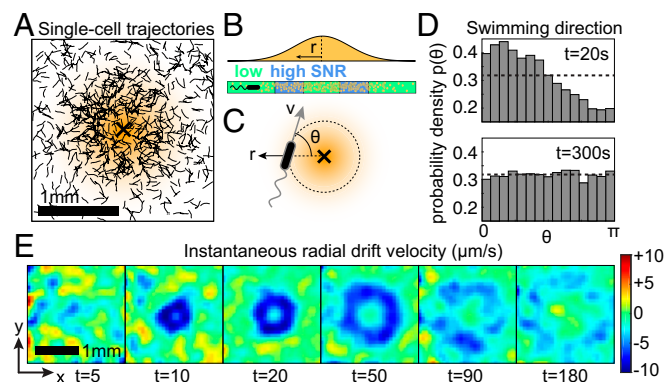
Fig. 2. Bacterial drift is confined to discrete regions in space and time where the SNR is sufficiently high. (A) Single-cell trajectories in the first 60 s following pulse release. (B) Schematic of the mean glutamate concentration as a function of the distance from the center of a pulse. Far from and near to the pulse center, the SNR is low. At an intermediate distance, concentration gradients are strong, and the gradient signal can emerge above noise. (C) The swimming velocity of each bacterium makes an angle \theta relative to the radial vector toward the pulse center. (D) Probability distribution, p(\theta) , of the swimming angle \theta within the region r \in [300\ \mu\text{m}, 400\ \mu\text{m}] . The dotted lines correspond to isotropic distributions (random swimming direction). A strong inward bias, E[\theta] < \pi/2 , is observed at t = 20 s. (E) Instantaneous radial drift velocity, v_{\text{drift}} , at various times following the pulse release.
